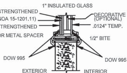
TYPICAL GLAZING DETAIL IMPACT RATED GLASS
