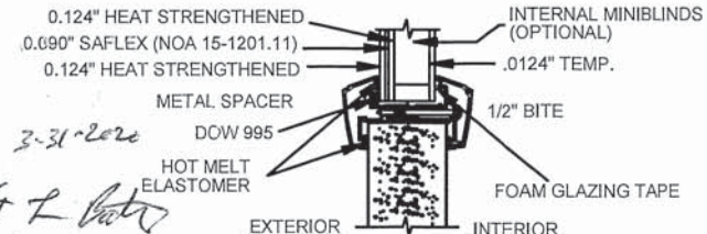
ALTERNATE GLAZING DETAIL IMPACT RATED GLASS
